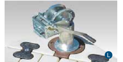
DEADWEIGHT WINCH INSERT Deadweight insert and cable winch added to our polyethylene pipe bracket allow easy dock adjustment for water fluctuations. Cable sold separately.
